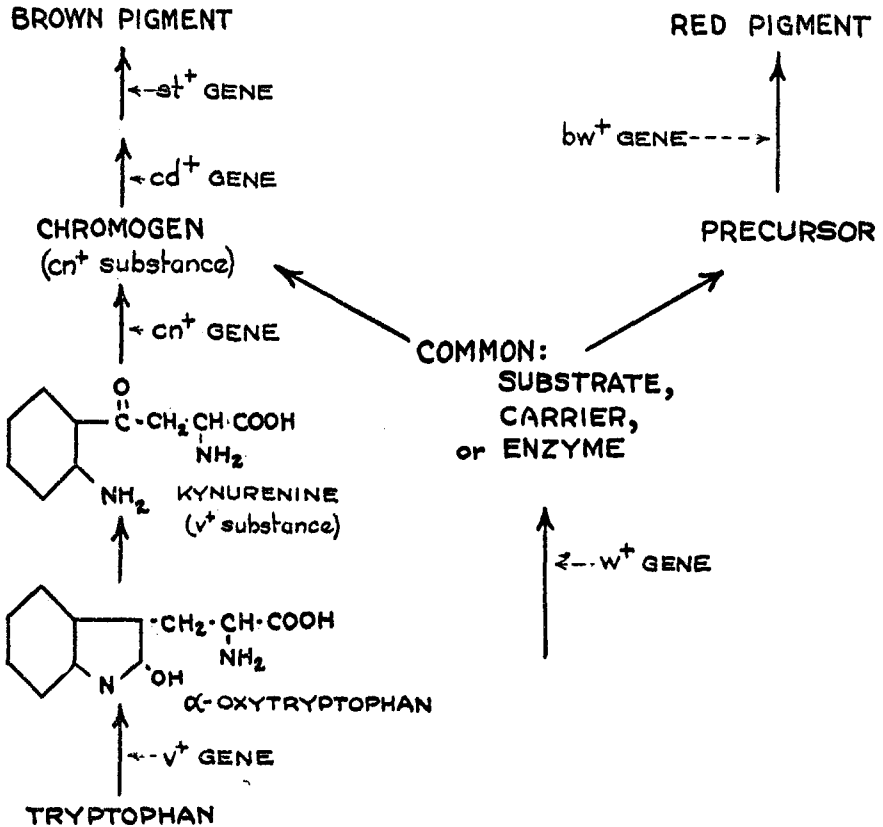
FIG. 3. Representation of insect eye-pigment development
