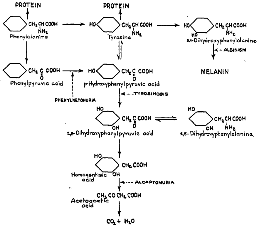
FIG. 1. Scheme of phenylalanine-tyrosine metabolism in man (based on interpretation given by Haldane (130)).
