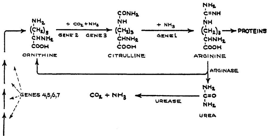
Fig. 6. Arginine cycle in Neurospora (after Srb and Horowitz (283))
