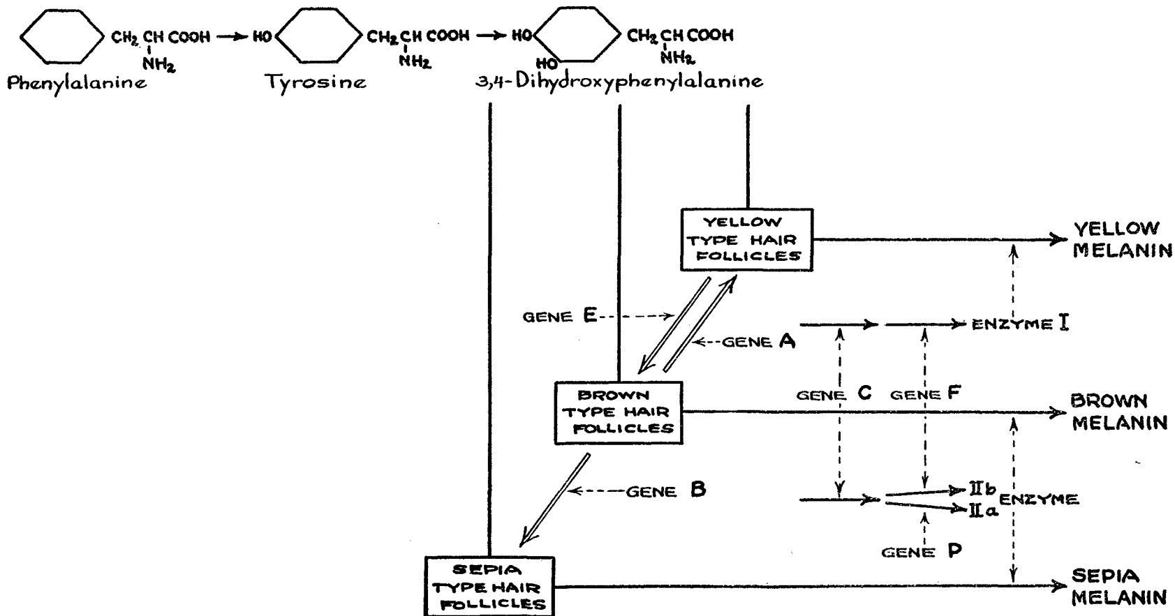
FIG. 2. Scheme of melanin synthesis in the guinea pig (based on work and interpretation of Wright (346, 347, 348, 350)). It is not certain that 3,4-dihydroxyphenylalanine is the common pigment precursor.
